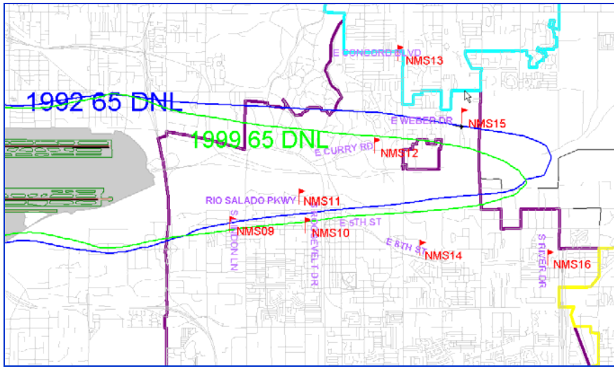
Eight of twenty fixed airport Noise Monitoring Sites (NMS) are located in Tempe
